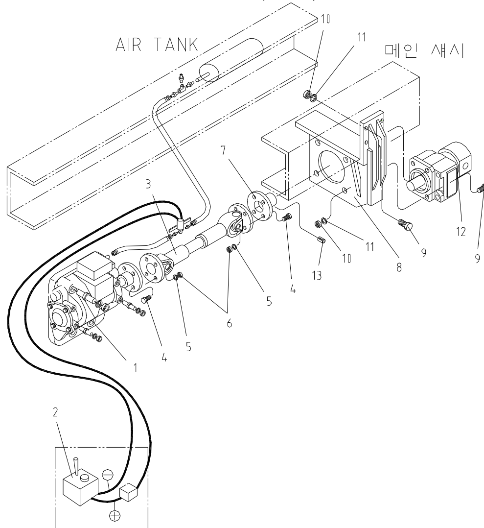
Fig. 8-1 SCS736 P.T.O &amp; PUMP PART(8TON)
