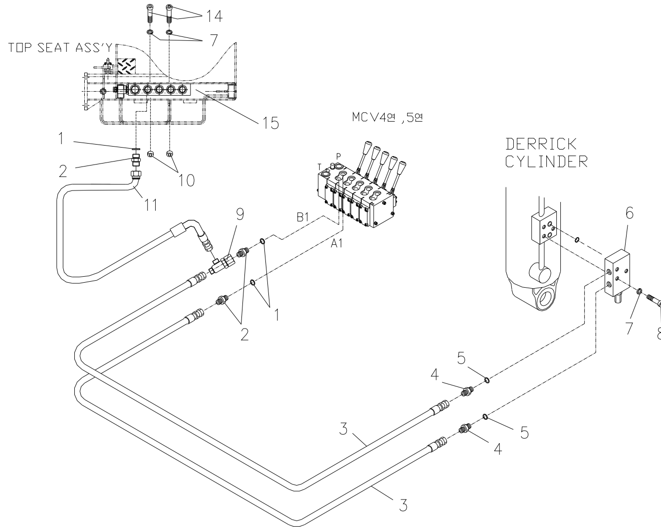
데릭 배관(탑형) Fig. 5-2 SCS736 DERRICK PIPING(TOP)
