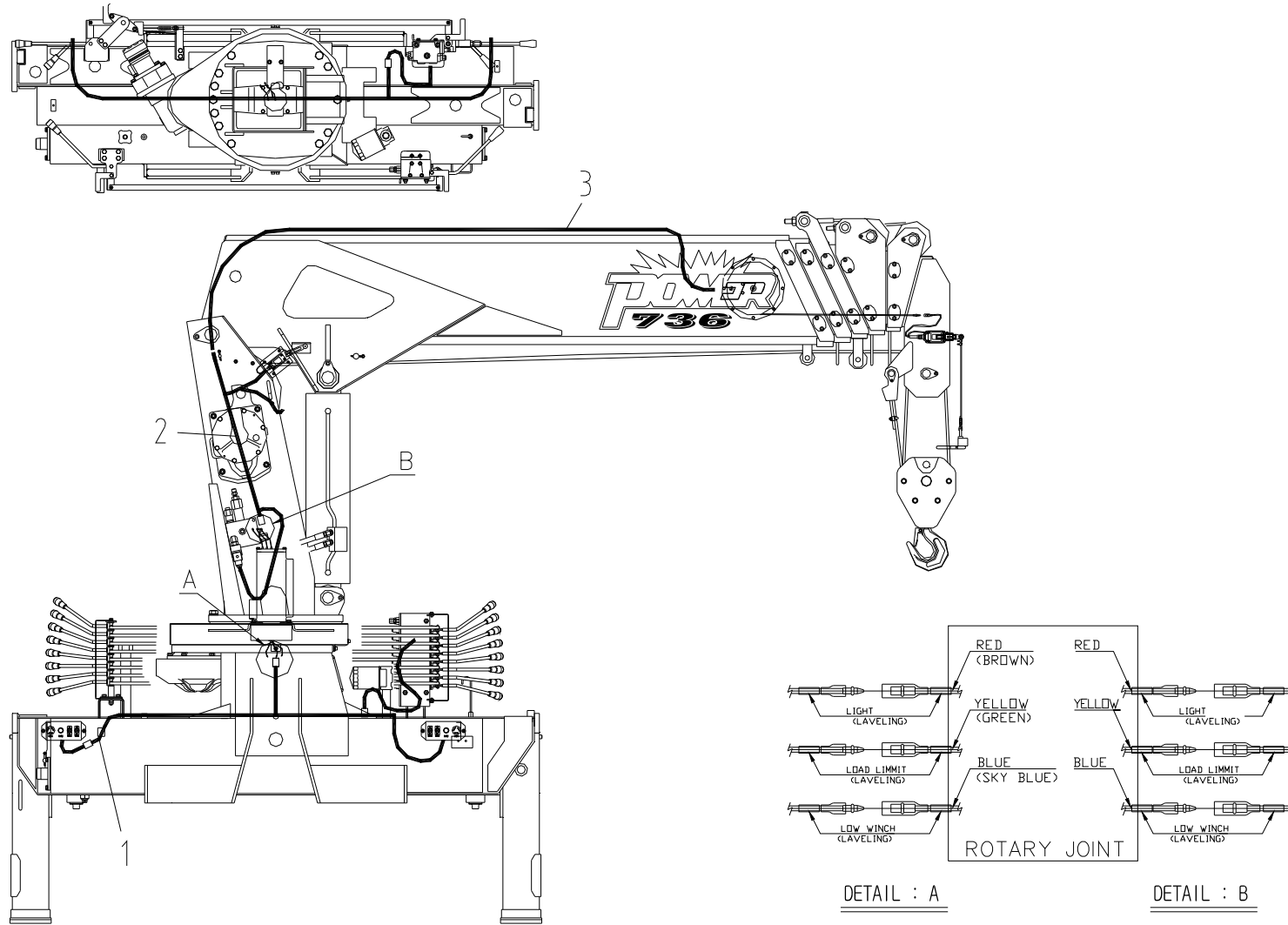
Fig. 10 SCS736 WIRING ASS'Y (STD)
